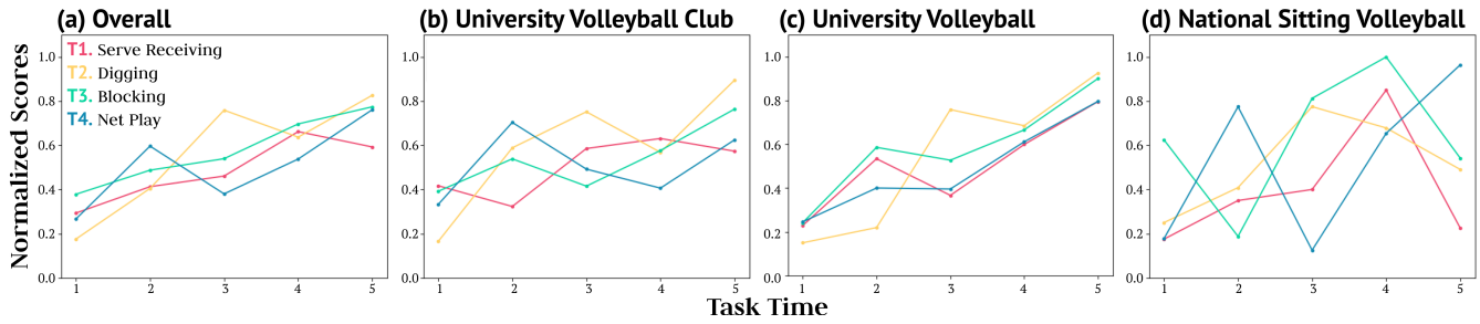
Fig. 6: Performance metrics over time for each participant group: (a) all participants, (b) University volleyball club team, (c) University volleyball team, and (d) National sitting volleyball team. The x-axis represents time in one-minute intervals, with '1' denoting the first minute and '5' the last, of the five-minute duration for each task as per Section 6.2. This normalized score progression demonstrates the enhancements or declines in skills such as serve receiving, digging, blocking, and net play over the course of the evaluation period.
