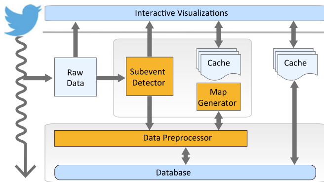
Fig. 2. Framework with four main components: Subevent detector, pre-processor, map generator, and interactive visualizations.
