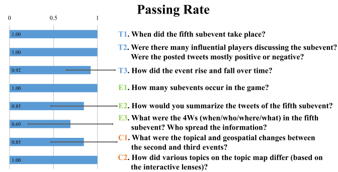
Fig. 10. Evaluation tasks and analysis of the passing rates.
