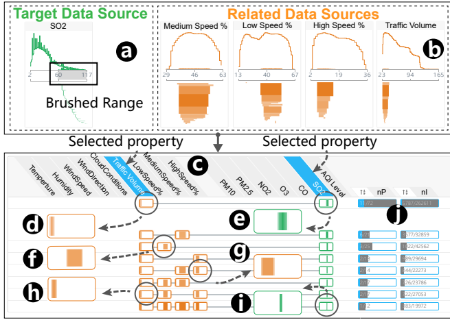
Fig. 9: Macro-level analysis of the co-occurrence patterns that are relevant to high \text{SO}_2 .
