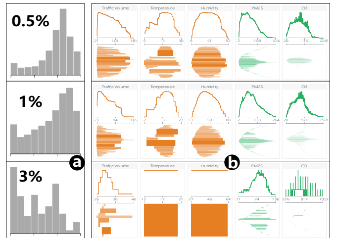
Fig. 8: Selecting proper parameters: (a) histograms showing the distribution of the normalized range widths and (b) statistical information for the co-occurrence coverage thresholds 0.5%, 1% and 3% in StatView.
